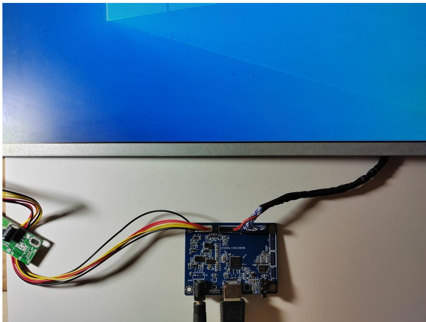
Figure 11: Connection method 2
