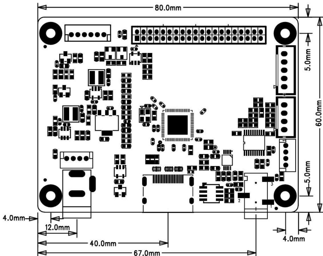
Figure 9: Mounting Dimensions
