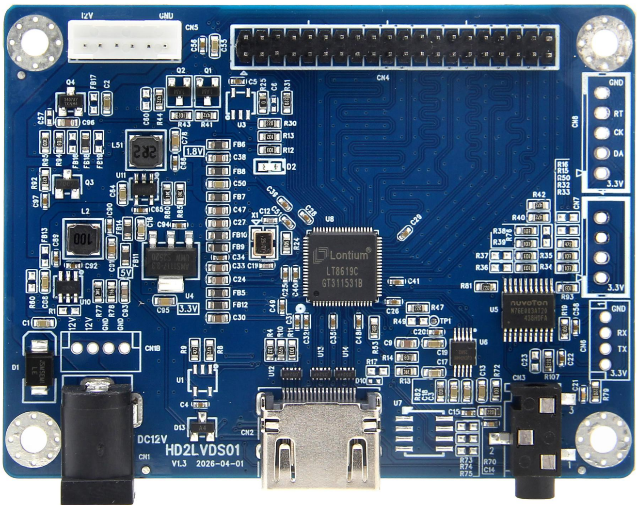
Figure 1: Board (8x6cm)
