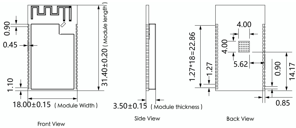
Figure 5: ESP32-WROVER Dimensions
